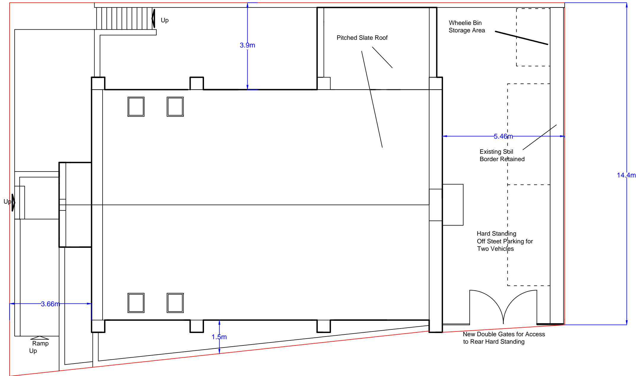
8DT2: 8 Derby Terrace Site Plan As Proposed Page 1 of 1, Scale 1:100 at A3
